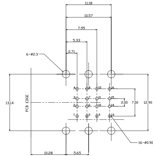
BOTTOM VIEW RECOMMENDED PCB LAYOUT
